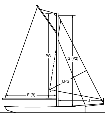
GAFF HEADED MAIN
