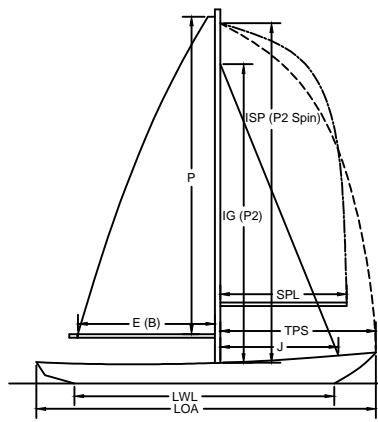
JIB HEADED MAIN
