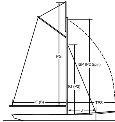
GAFF HEADED MAIN W / TOPSAIL
