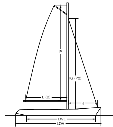
SQUARE HEADED MAIN
