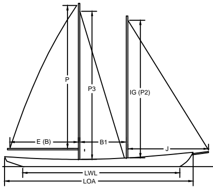
STAYSAIL SCHOONER A
