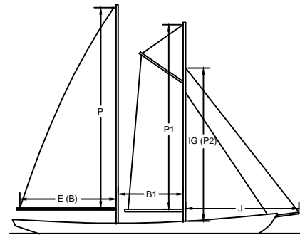
GAFF FORESAIL W / TOPSAIL
