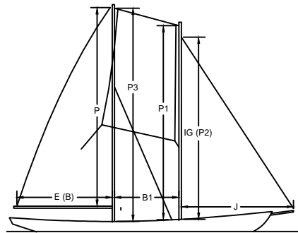
STAYSAIL SCHOONER B
