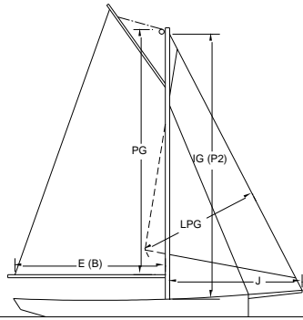
GAUFF HEADED MAIN
