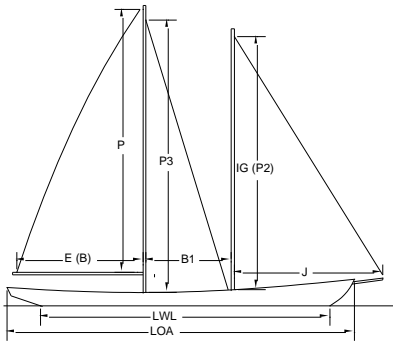
STAYSAIL SCHOONER
