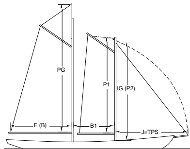
GAUFF FORESAIL
