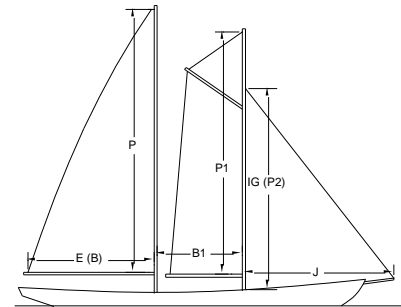
GAUFF FORESAIL W / TOPSAIL
